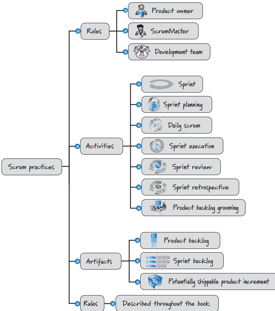
FIGURE 2.1 Scrum practices
